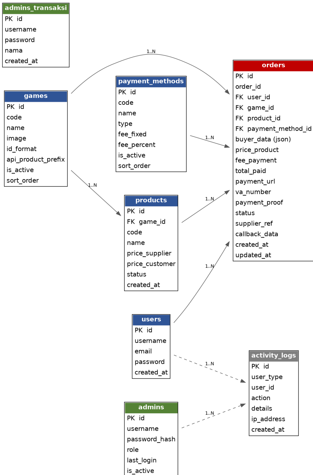
Gambar 3.1 Entity Relationship Diagram (ERD) basis data TopUpKu
